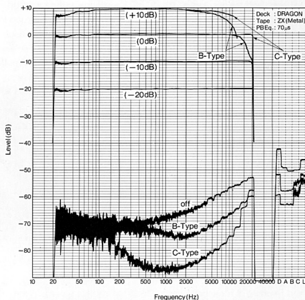
Record/Play Frequency Response and Noise Spectrum Analysis of the DRAGON
